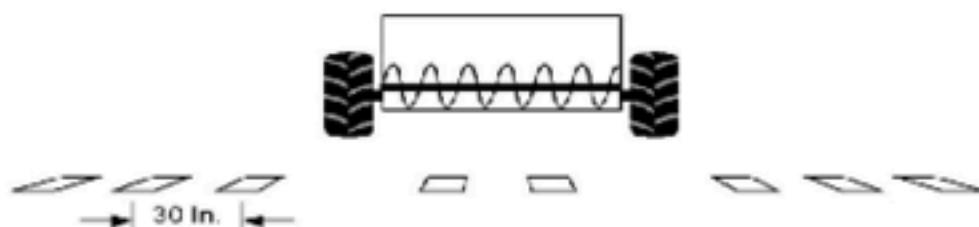
Figure 1. Common sheet layout pattern for a rear-beater spreader.
